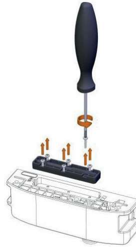
Phase 2. Unscrew the 6 fixing screws and lift the plate
