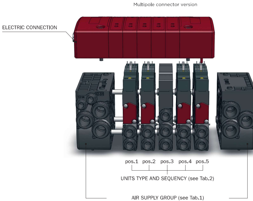
Single cabling with connector version
